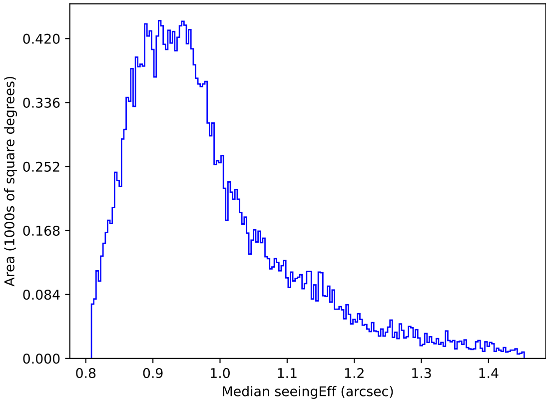
weather_cloudso30v3.4_10yrs Yr 1 all bands: Median seeingEff
