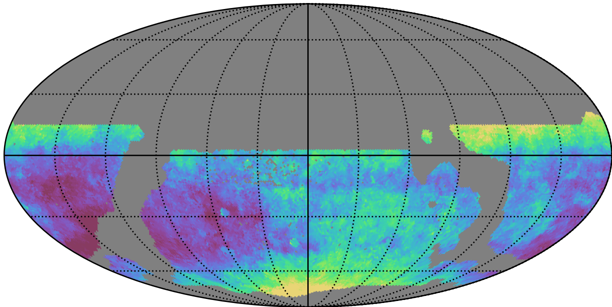
weather_cloudso30v3.4_10yrs WFD z band: Median seeingEff
