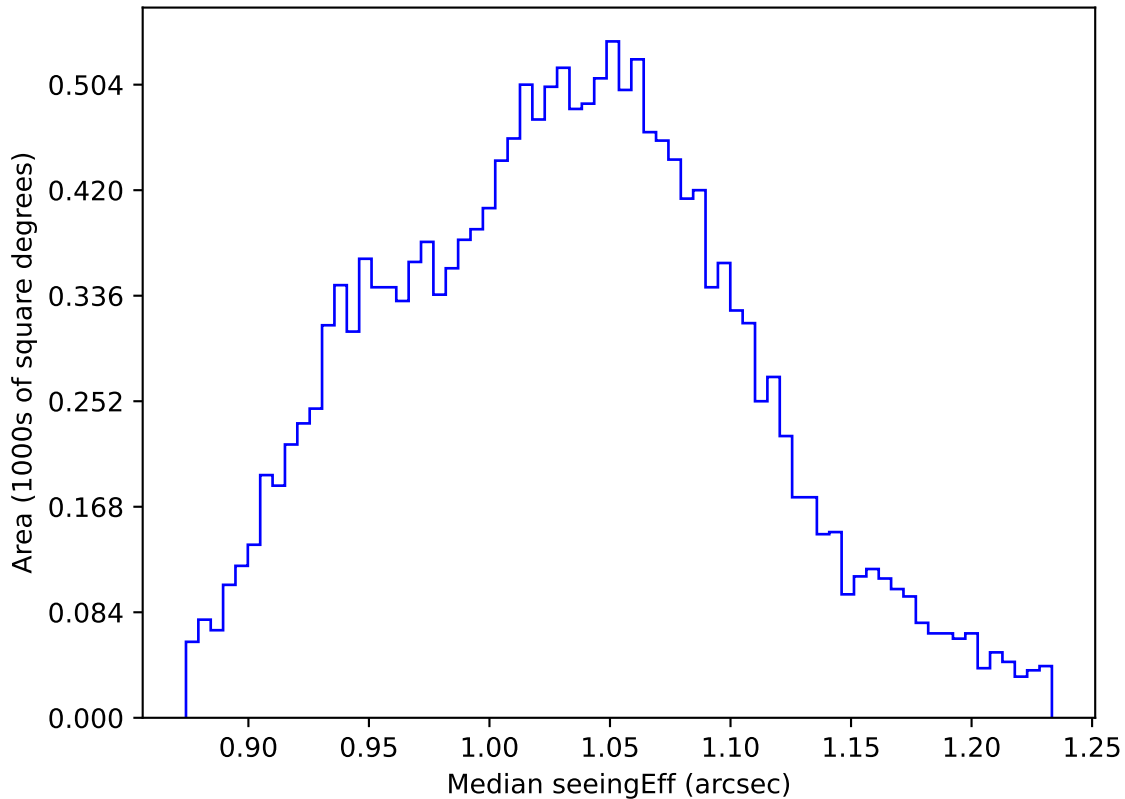
weather_cloudso30v3.4_10yrs WFD z band: Median seeingEff
