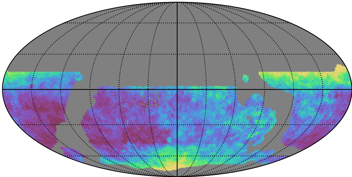
weather_cloudso30v3.4_10yrs WFD y band: Median seeingEff
