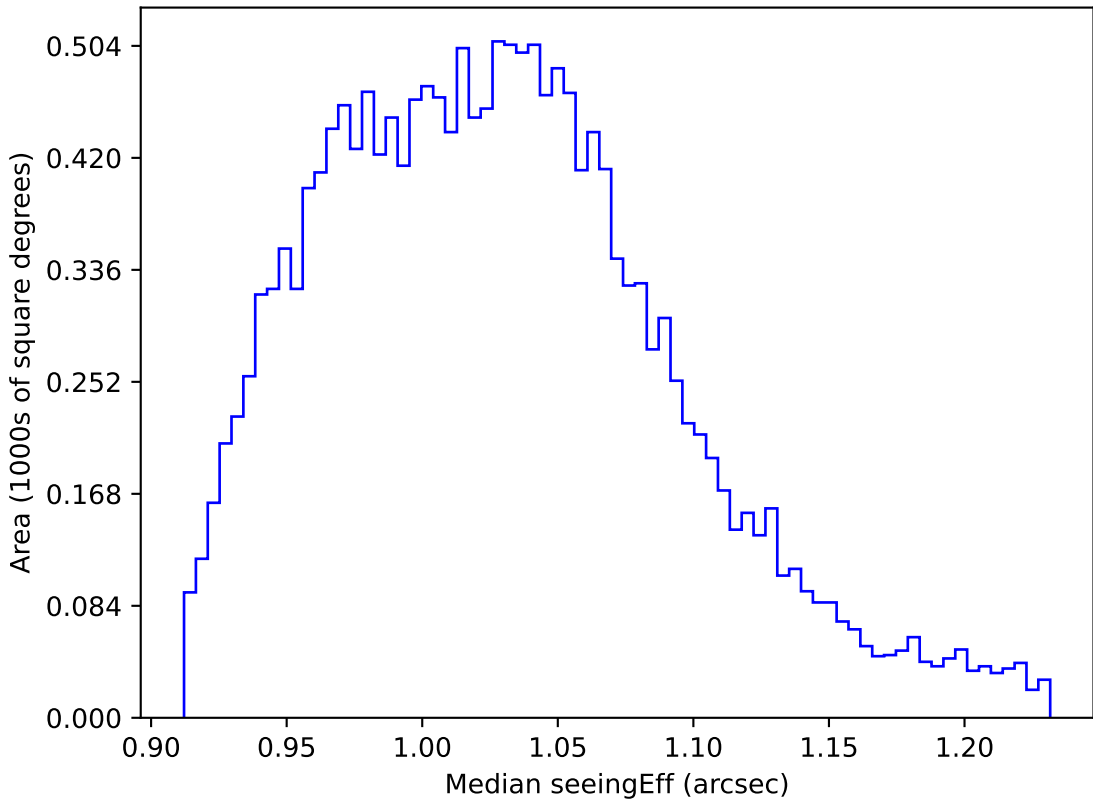
weather_cloudso30v3.4_10yrs WFD y band: Median seeingEff
