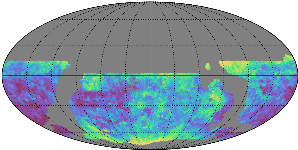
weather_cloudso30v3.4_10yrs WFD u band: Median seeingEff
