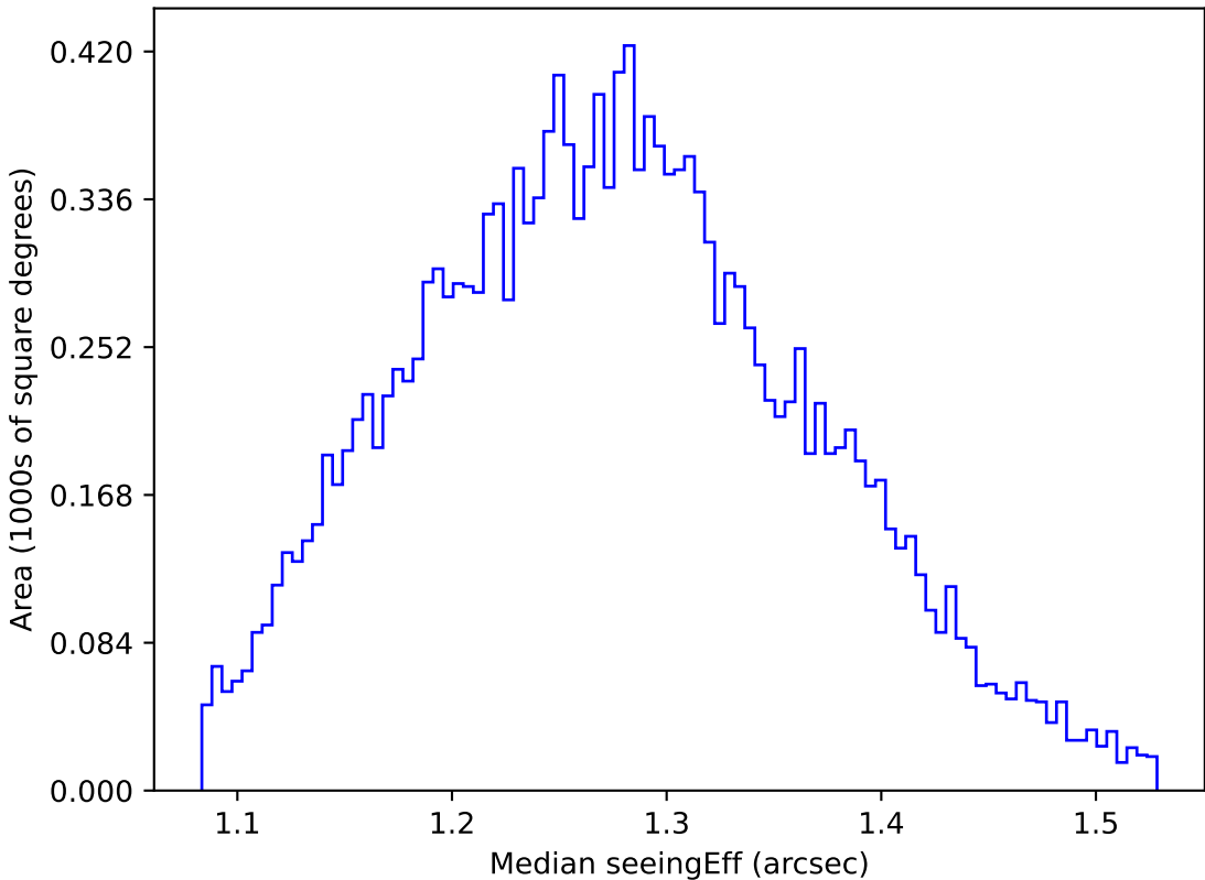
weather_cloudso30v3.4_10yrs WFD u band: Median seeingEff
