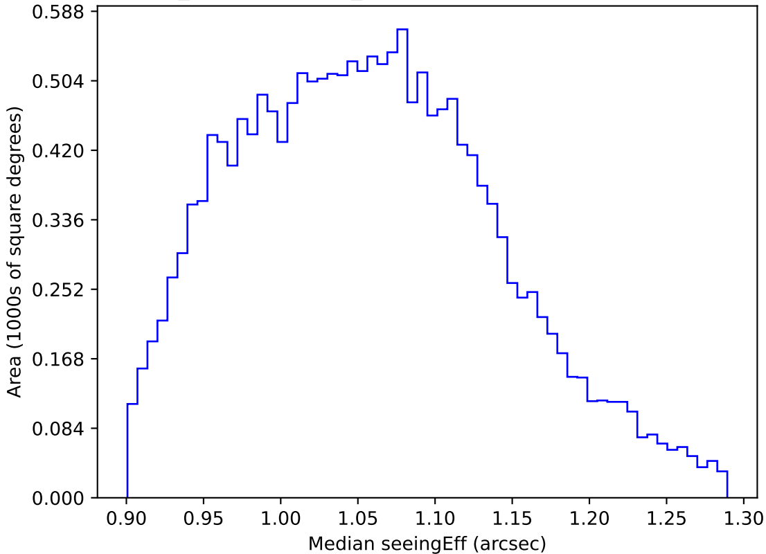
weather_cloudso30v3.4_10yrs WFD r band: Median seeingEff
