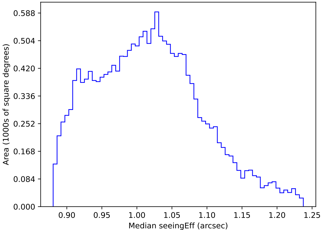
weather_cloudso30v3.4_10yrs WFD i band: Median seeingEff
