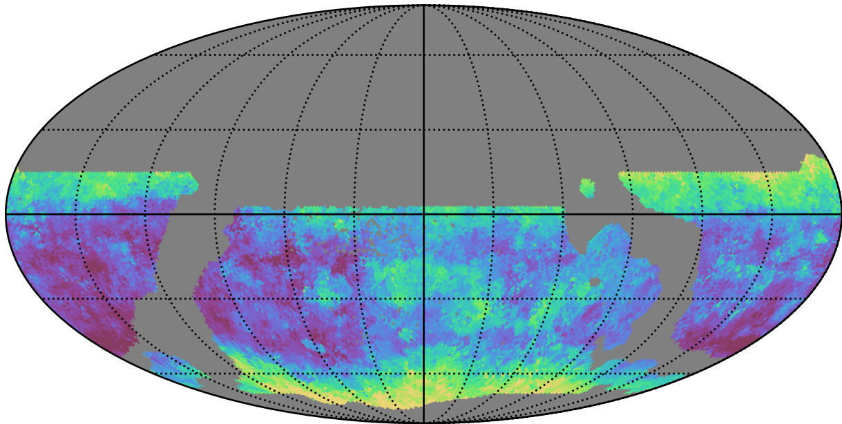
weather_cloudso30v3.4_10yrs WFD g band: Median seeingEff
