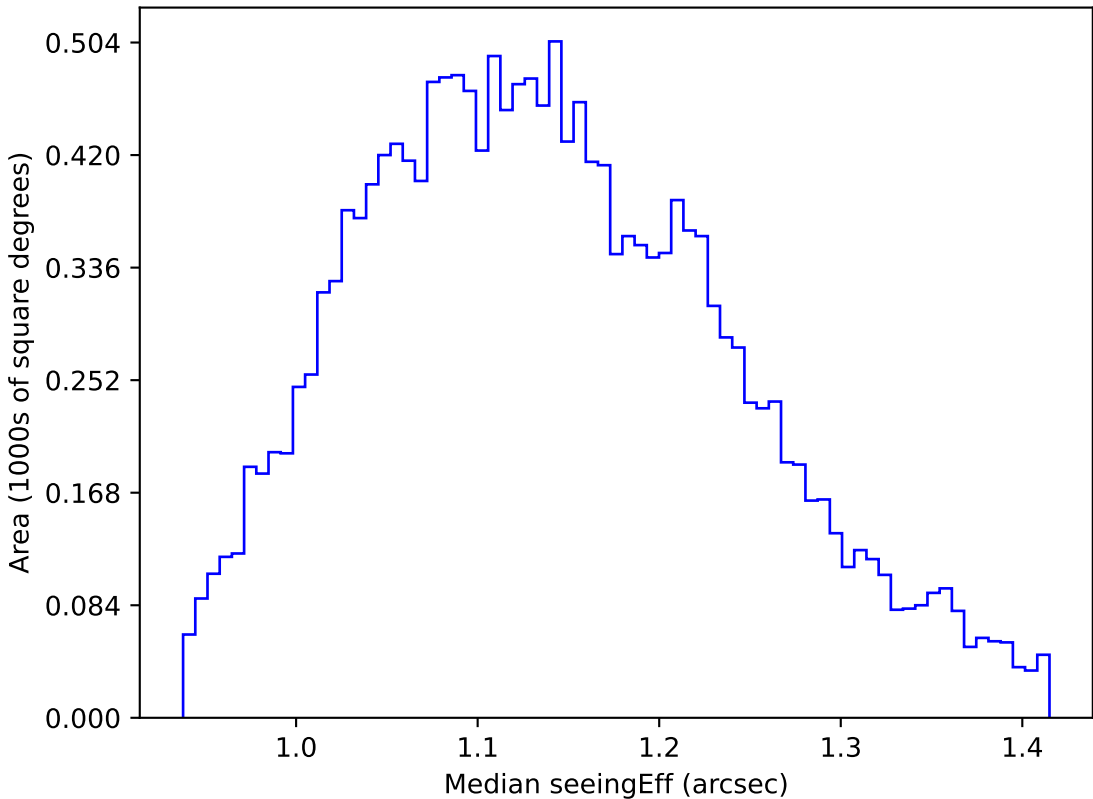
weather_cloudso30v3.4_10yrs WFD g band: Median seeingEff
