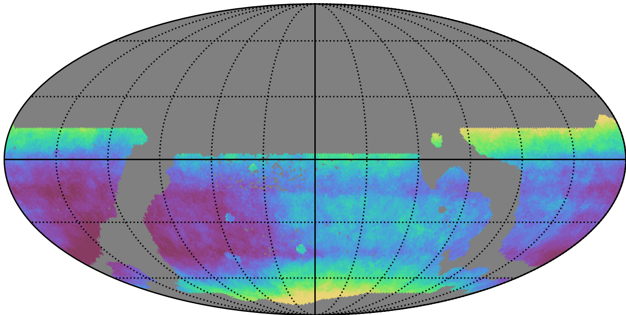
weather_cloudso30v3.4_10yrs WFD all bands: Median seeingEff
