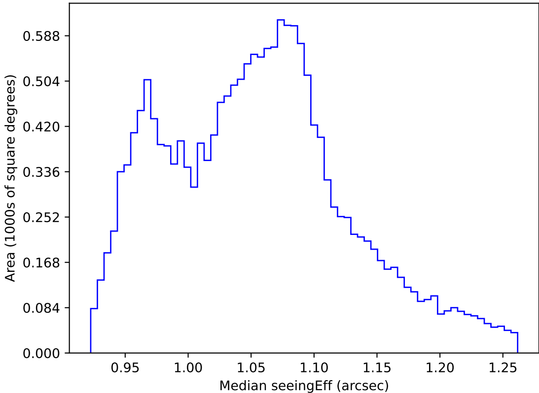
weather_cloudso30v3.4_10yrs WFD all bands: Median seeingEff
