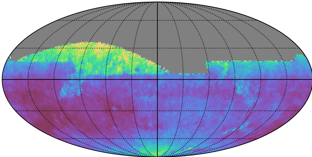
weather_cloudso30v3.4_10yrs All sky z band: Median seeingEff
