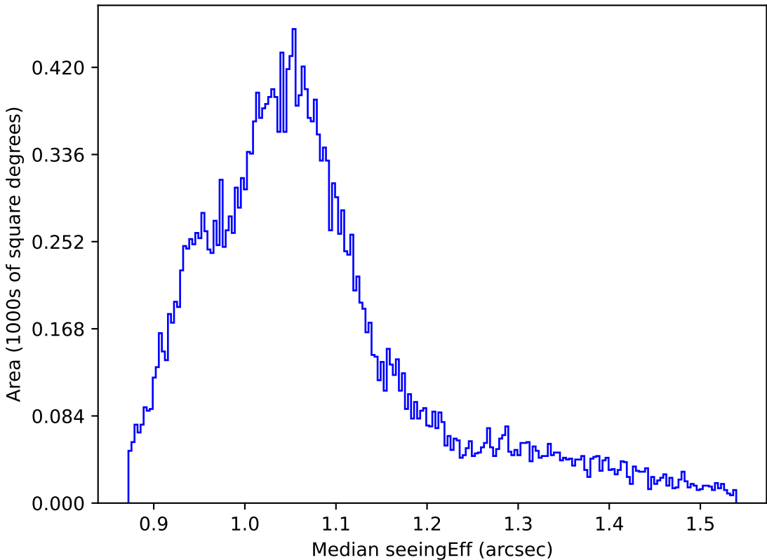
weather_cloudso30v3.4_10yrs All sky z band: Median seeingEff
