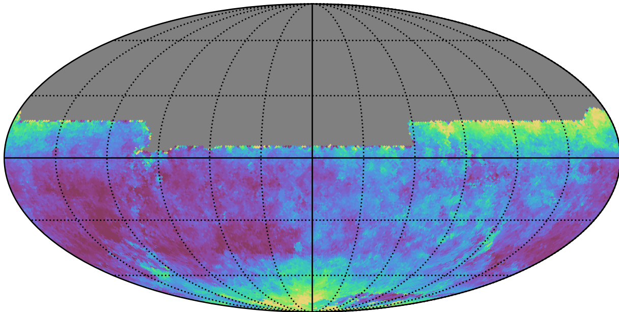
weather_cloudso30v3.4_10yrs All sky y band: Median seeingEff
