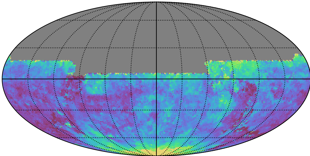
weather_cloudso30v3.4_10yrs All sky u band: Median seeingEff
