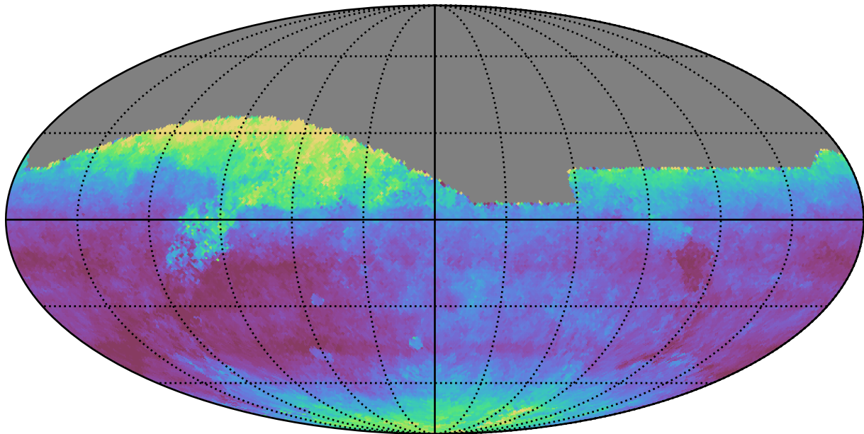
weather_cloudso30v3.4_10yrs All sky r band: Median seeingEff
