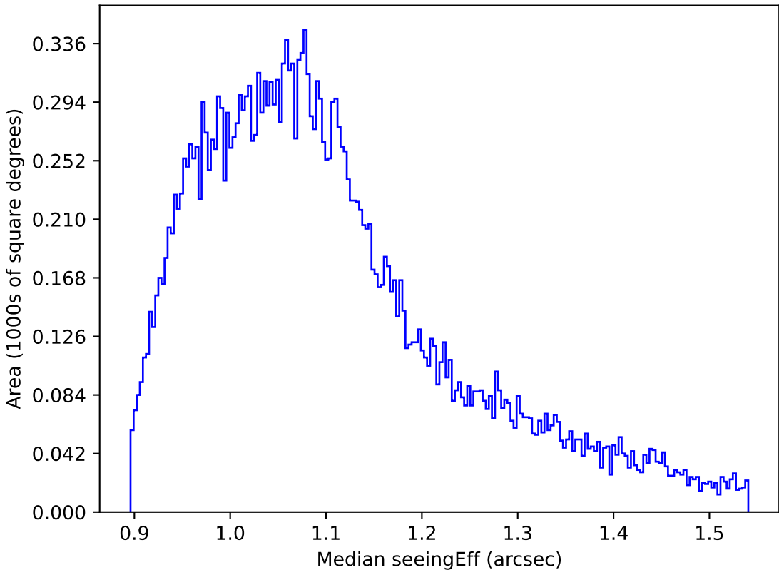
weather_cloudso30v3.4_10yrs All sky r band: Median seeingEff
