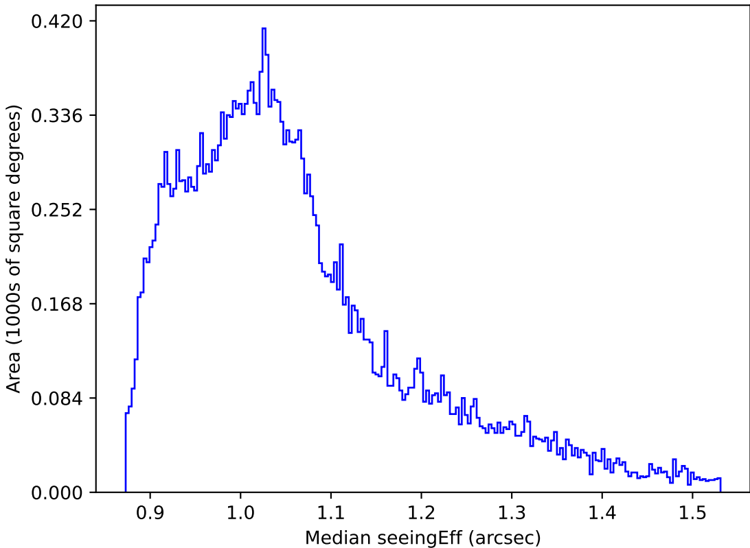
weather_cloudso30v3.4_10yrs All sky i band: Median seeingEff
