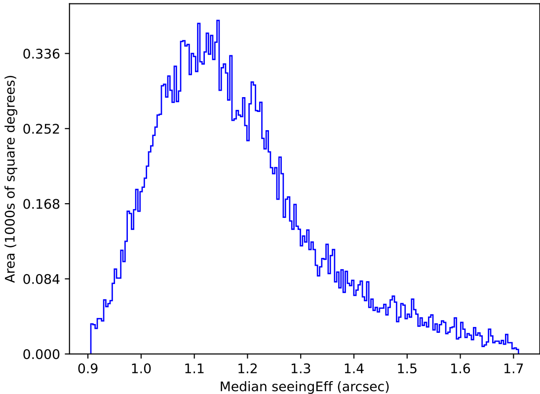
weather_cloudso30v3.4_10yrs All sky g band: Median seeingEff
