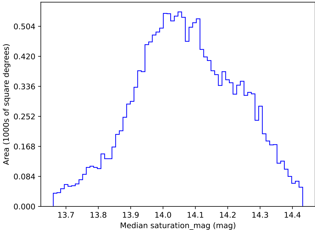
weather_cloudso30v3.4_10yrs WFD z band: Median saturation_mag
