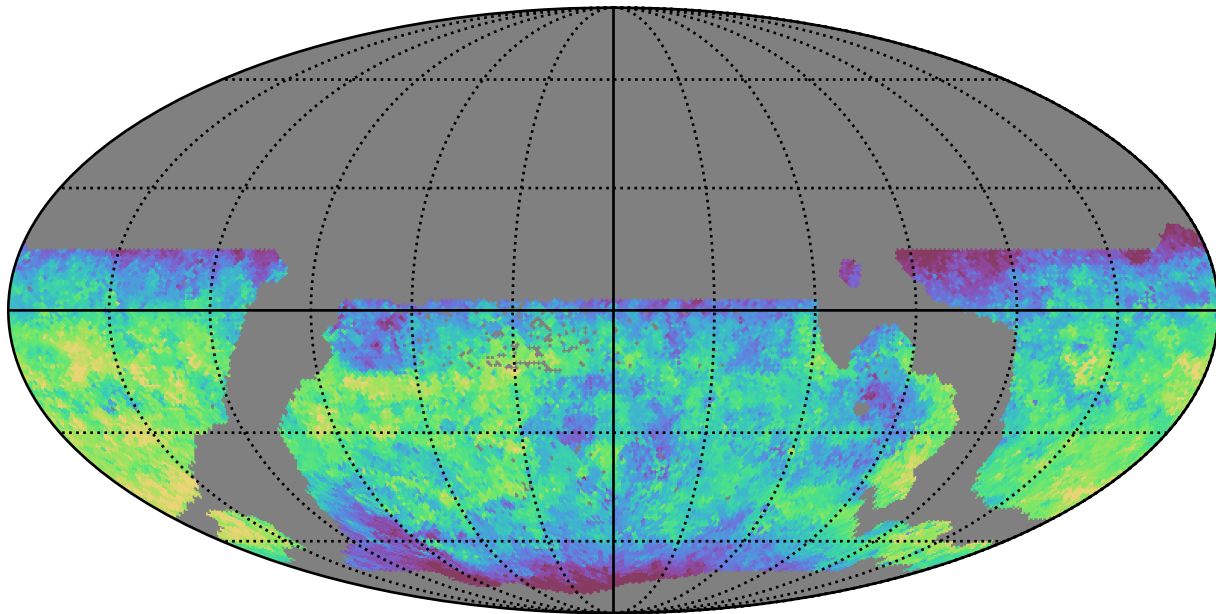
weather_cloudso30v3.4_10yrs WFD u band: Median saturation_mag
