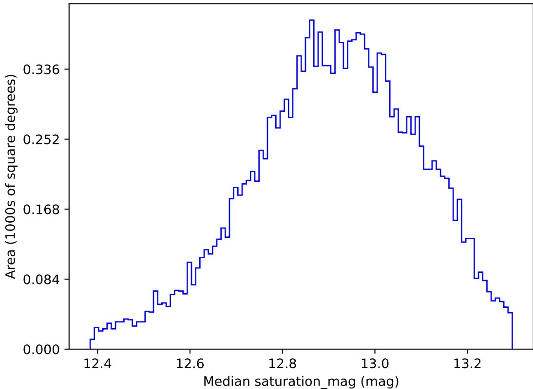
weather_cloudso30v3.4_10yrs WFD u band: Median saturation_mag
