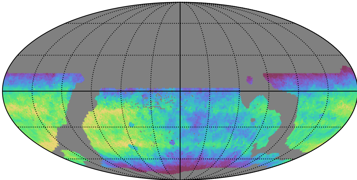
weather_cloudso30v3.4_10yrs WFD r band: Median saturation_mag
