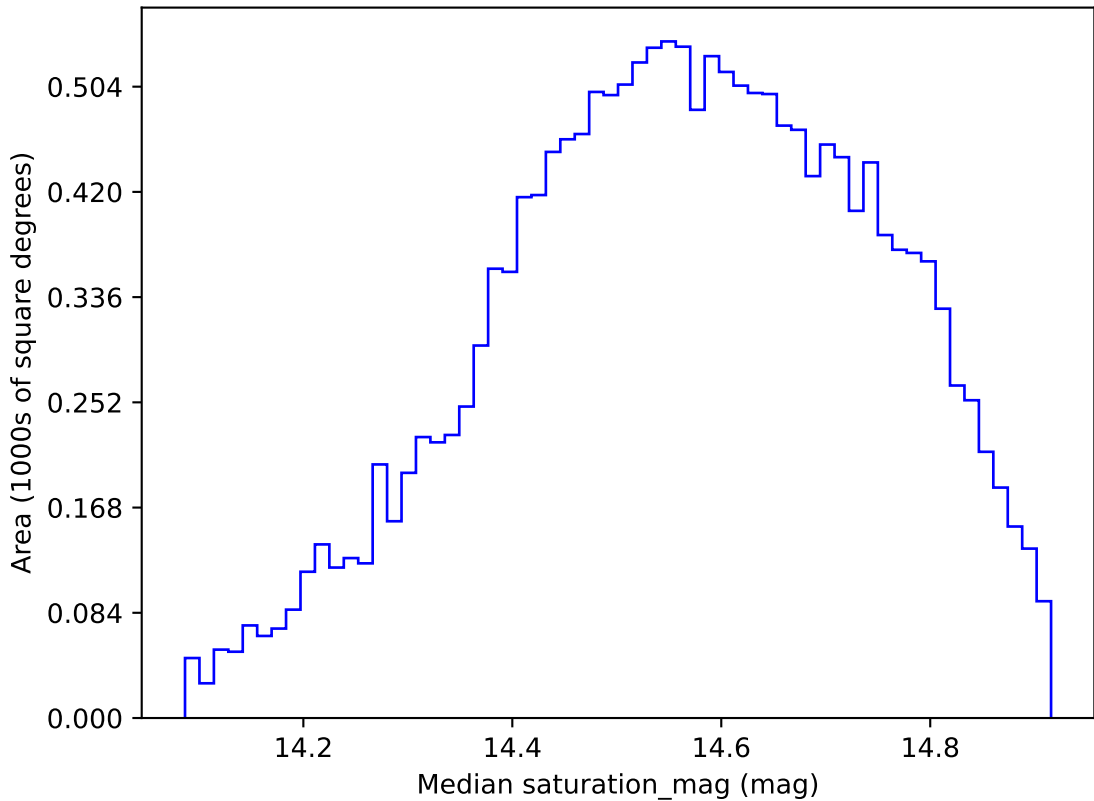
weather_cloudso30v3.4_10yrs WFD r band: Median saturation_mag
