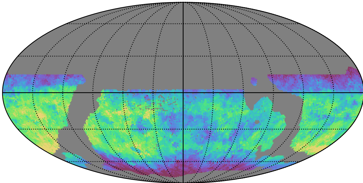
weather_cloudso30v3.4_10yrs WFD g band: Median saturation_mag
