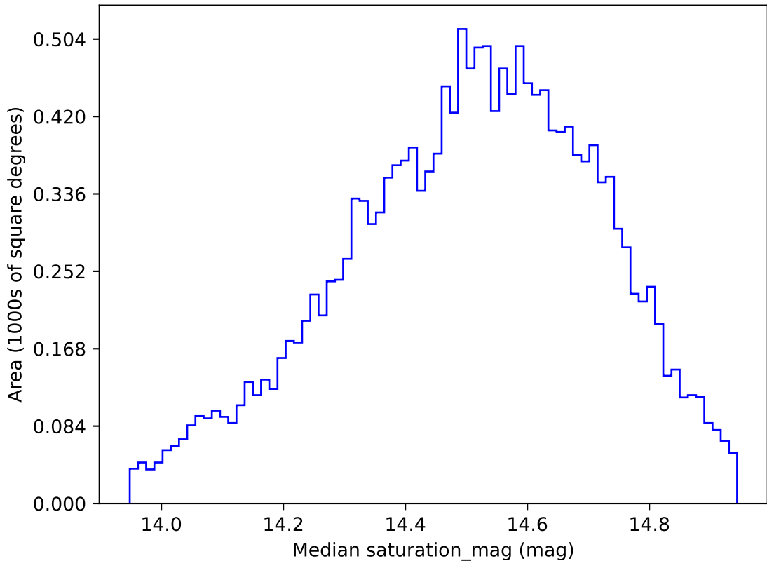
weather_cloudso30v3.4_10yrs WFD g band: Median saturation_mag
