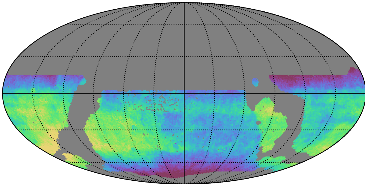
weather_cloudso30v3.4_10yrs WFD all bands: Median saturation_mag
