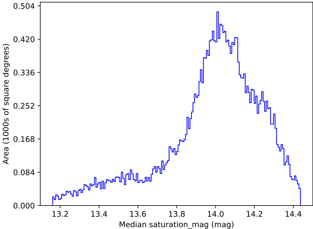
weather_cloudso30v3.4_10yrs All sky z band: Median saturation_mag
