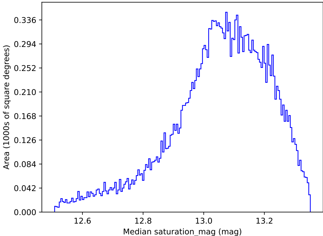
weather_cloudso30v3.4_10yrs All sky y band: Median saturation_mag
