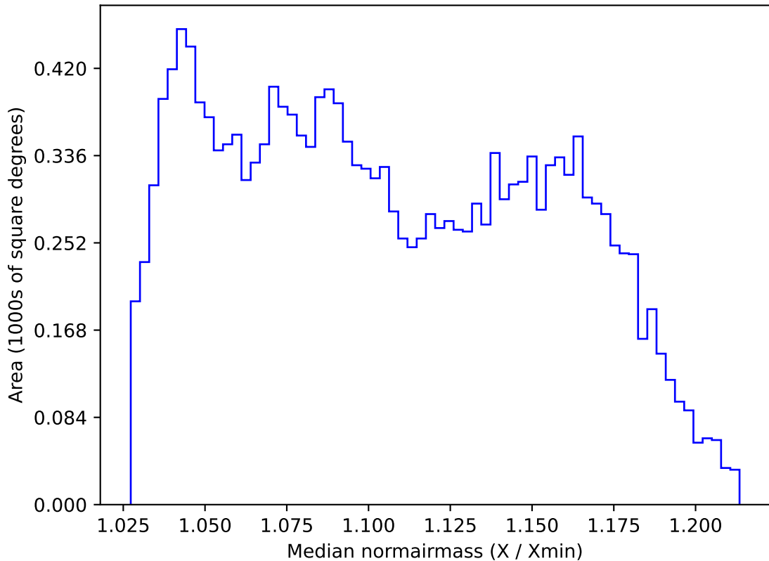
weather_cloudso30v3.4_10yrs WFD z band: Median normairmass
