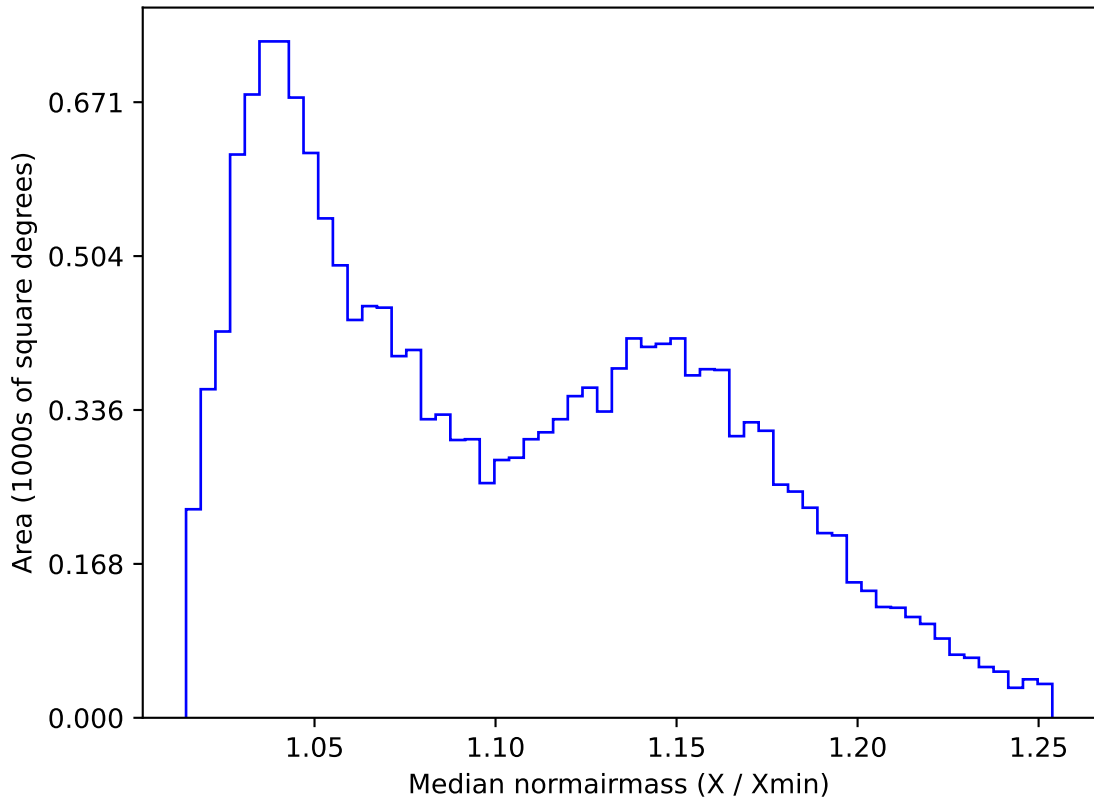
weather_cloudso30v3.4_10yrs WFD u band: Median normairmass
