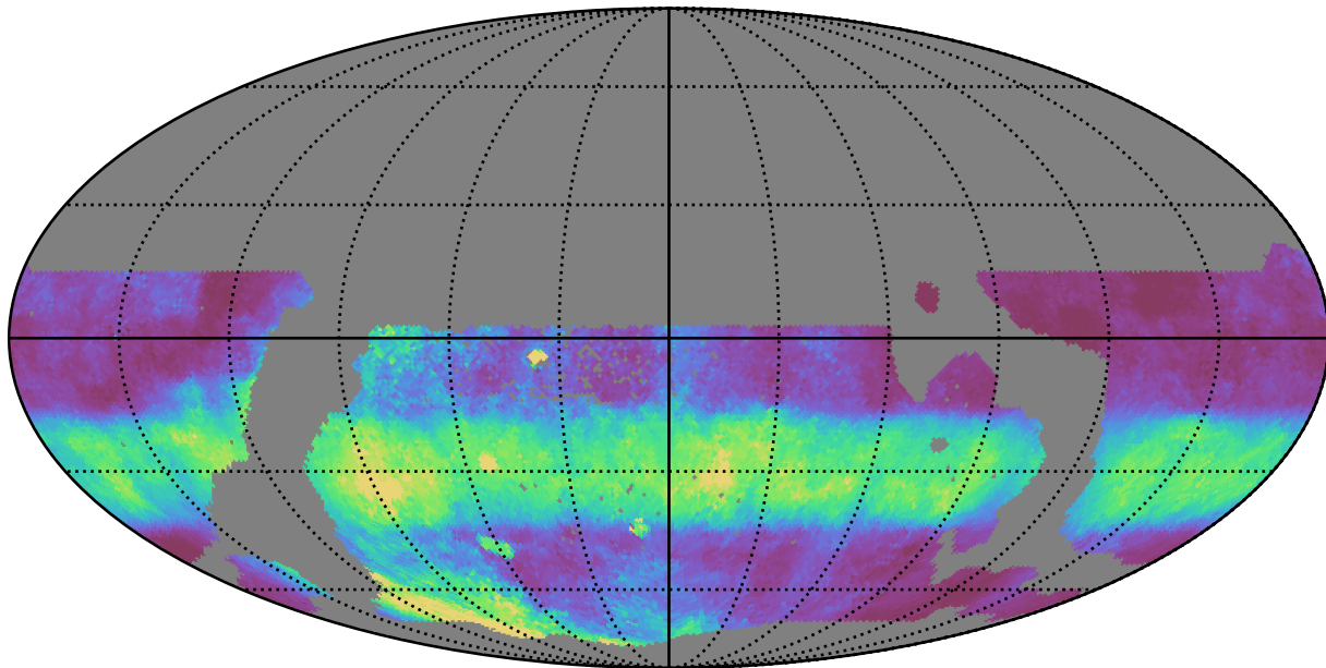
weather_cloudso30v3.4_10yrs WFD r band: Median normairmass
