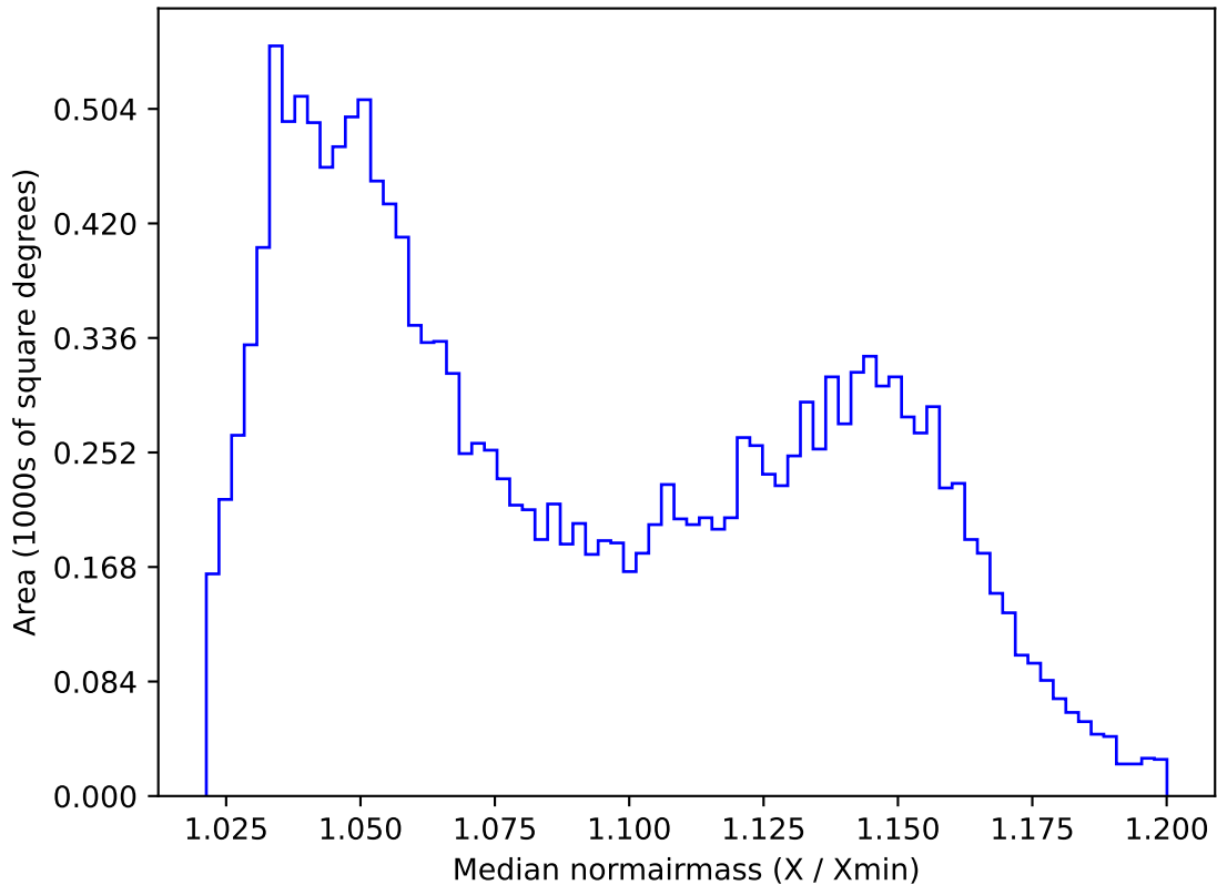
weather_cloudso30v3.4_10yrs WFD r band: Median normairmass
