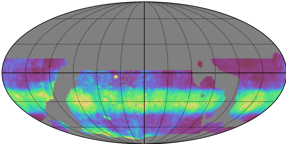
weather_cloudso30v3.4_10yrs WFD i band: Median normairmass
