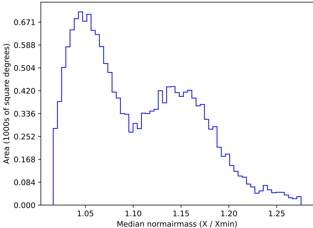
weather_cloudso30v3.4_10yrs WFD g band: Median normairmass
