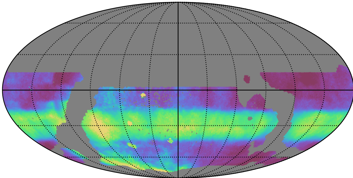
weather_cloudso30v3.4_10yrs WFD all bands: Median normairmass
