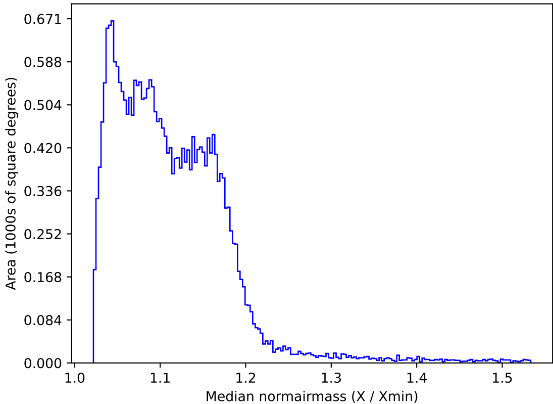
weather_cloudso30v3.4_10yrs All sky z band: Median normairmass
