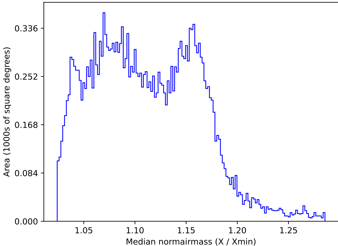
weather_cloudso30v3.4_10yrs All sky y band: Median normairmass
