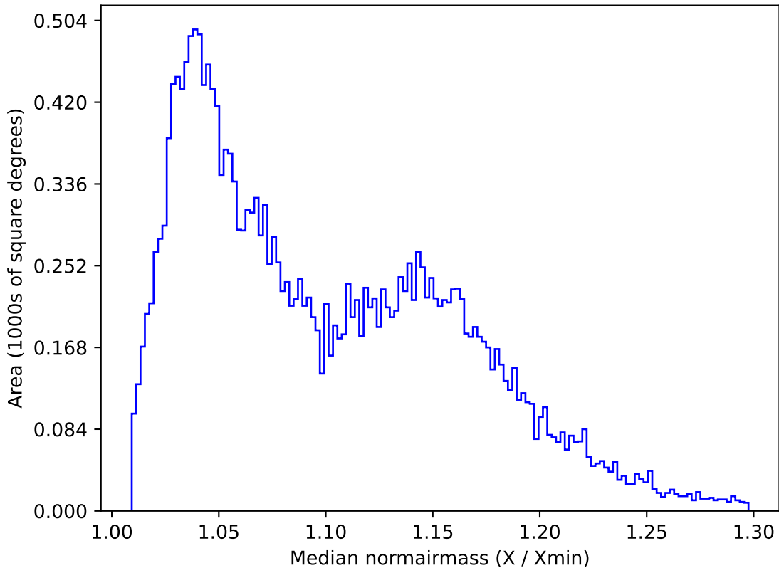
weather_cloudso30v3.4_10yrs All sky u band: Median normairmass
