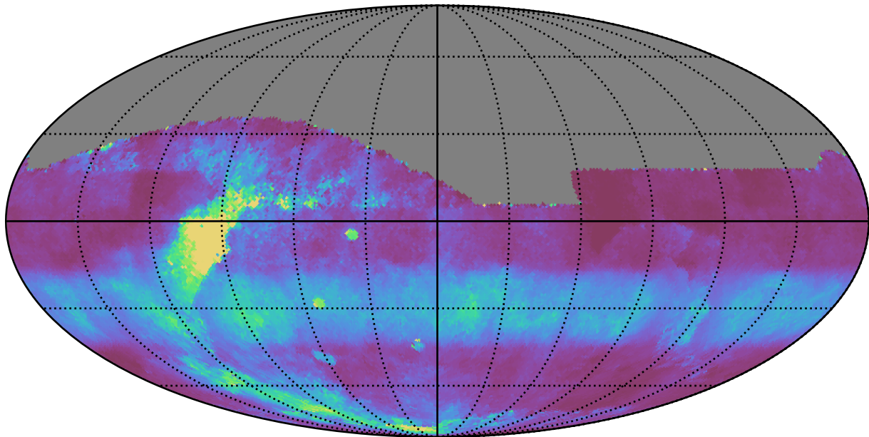
weather_cloudso30v3.4_10yrs All sky r band: Median normairmass
