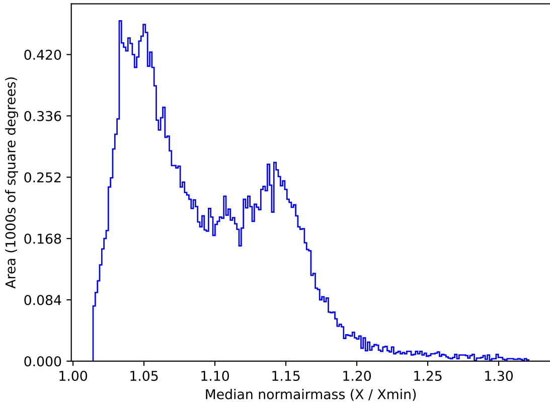
weather_cloudso30v3.4_10yrs All sky r band: Median normairmass
