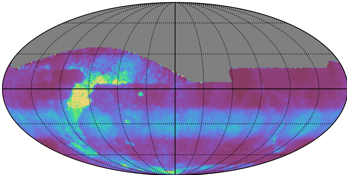
weather_cloudso30v3.4_10yrs All sky i band: Median normairmass
