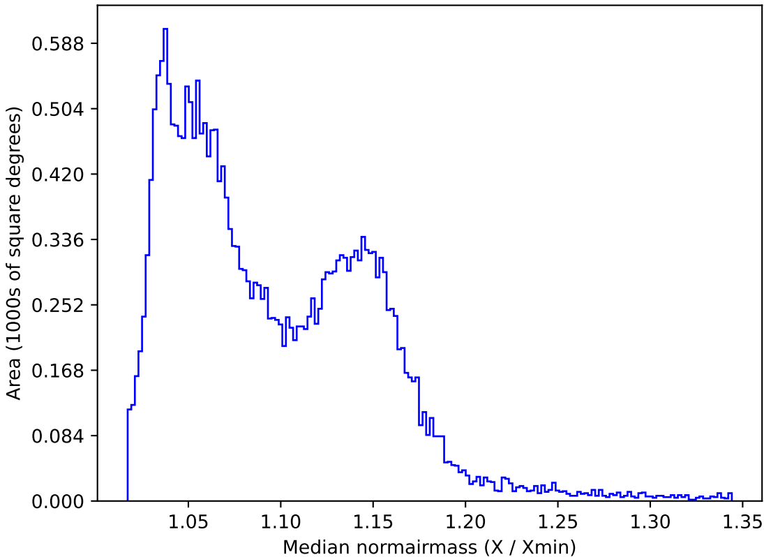
weather_cloudso30v3.4_10yrs All sky i band: Median normairmass
