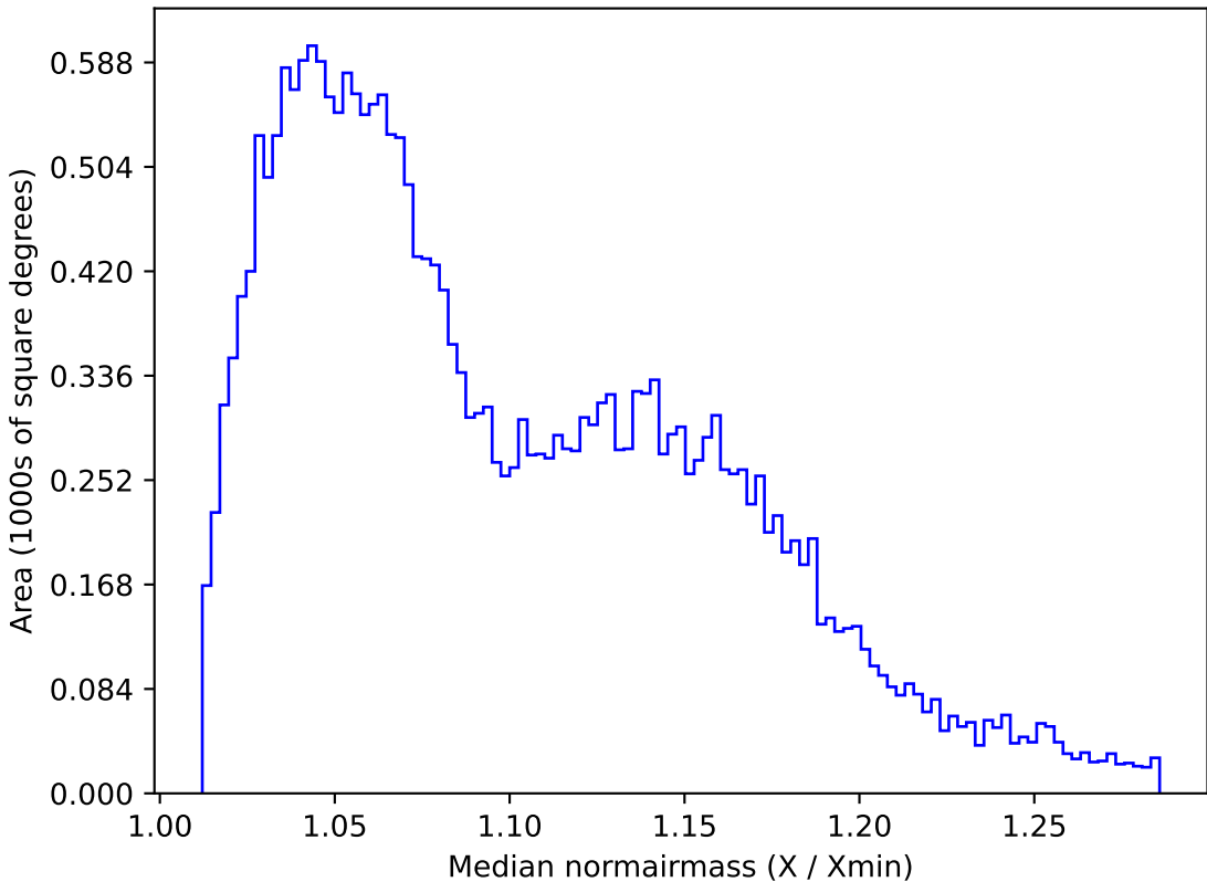
weather_cloudso30v3.4_10yrs All sky g band: Median normairmass
