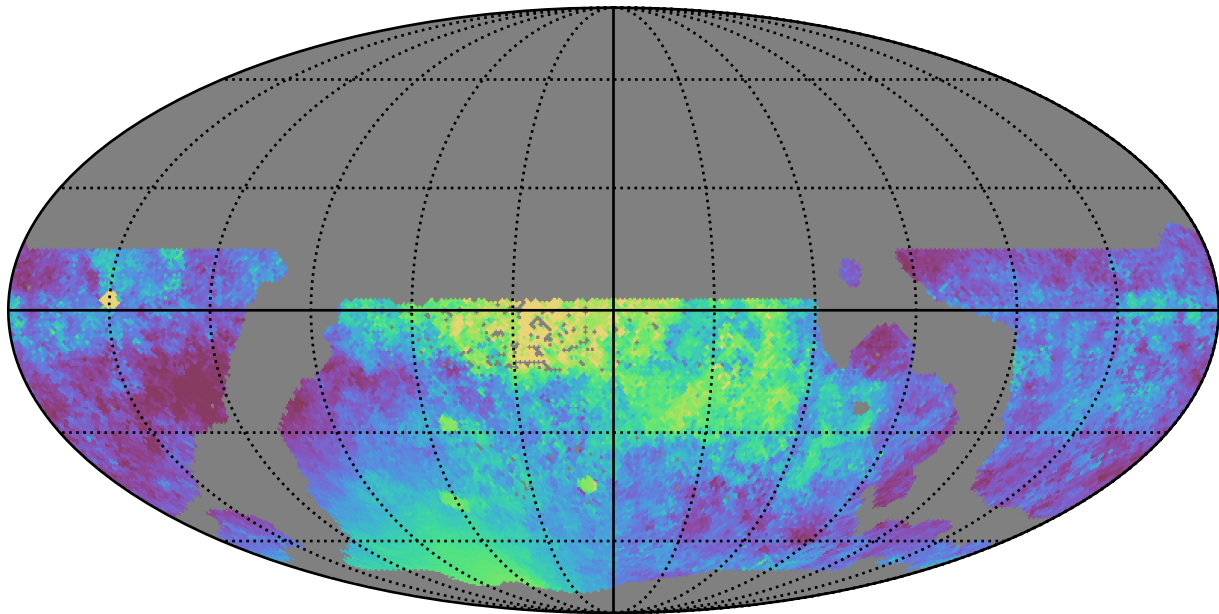
weather_cloudso30v3.4_10yrs WFD z band: Median moonDistance
