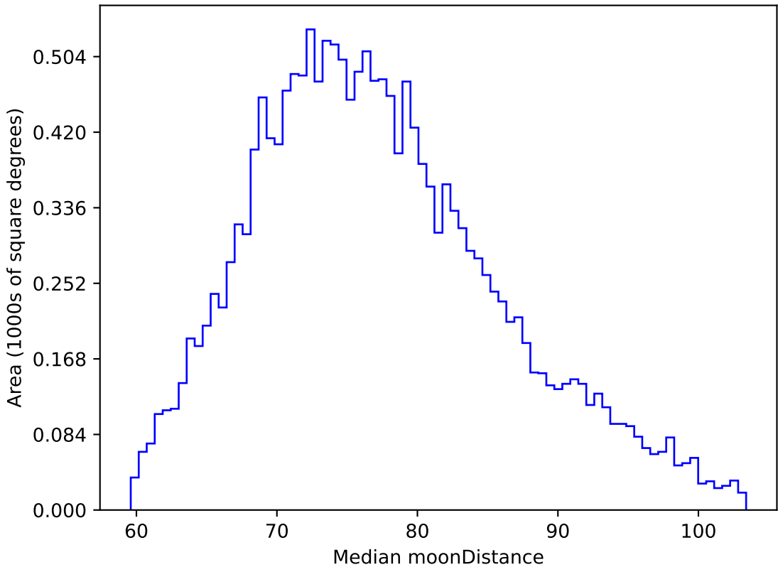
weather_cloudso30v3.4_10yrs WFD z band: Median moonDistance
