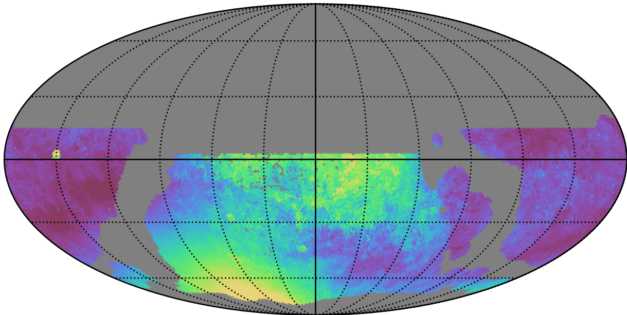
weather_cloudso30v3.4_10yrs WFD y band: Median moonDistance
