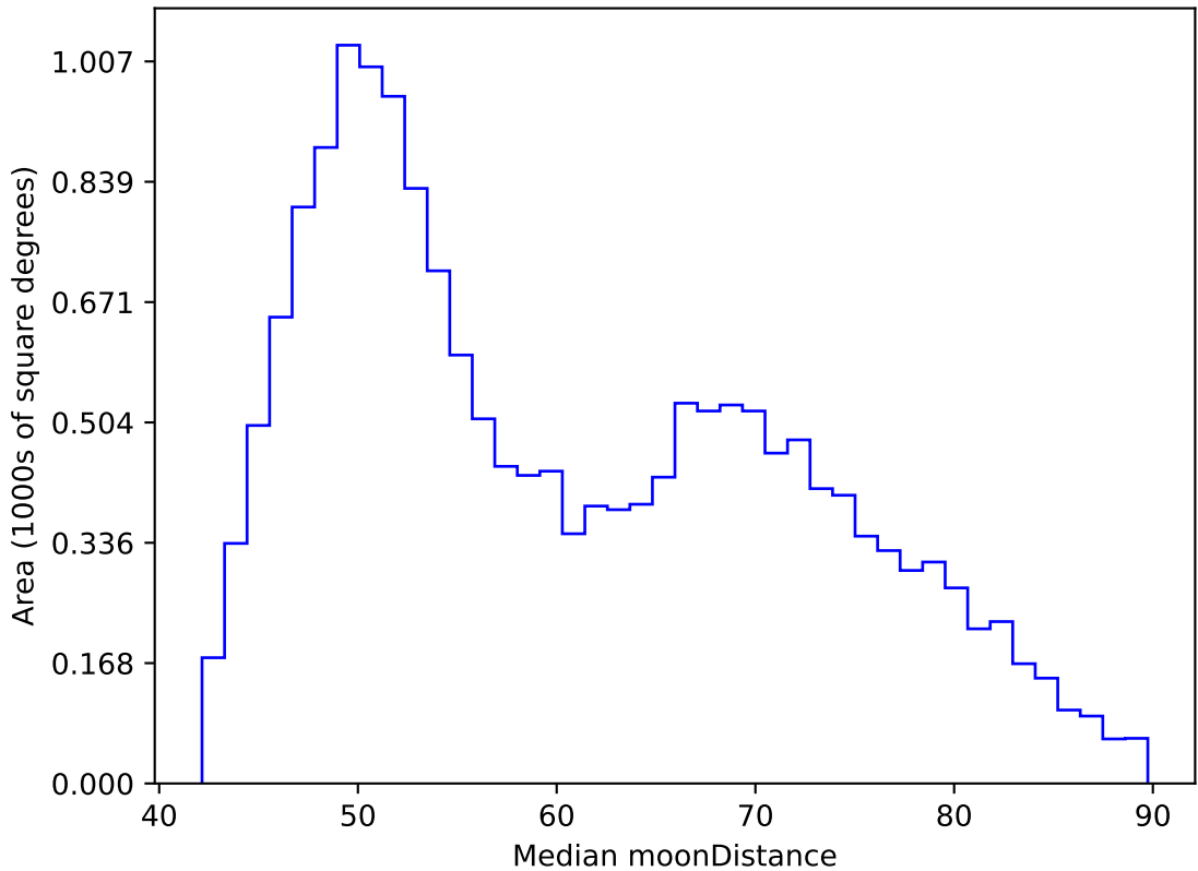
weather_cloudso30v3.4_10yrs WFD y band: Median moonDistance
